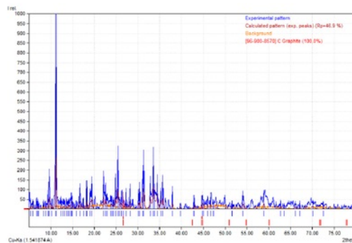
FIG. 3. Diffractogram of synthesized GO.
