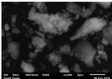
FIG. 5. SEM picture of GO after synthesis.
