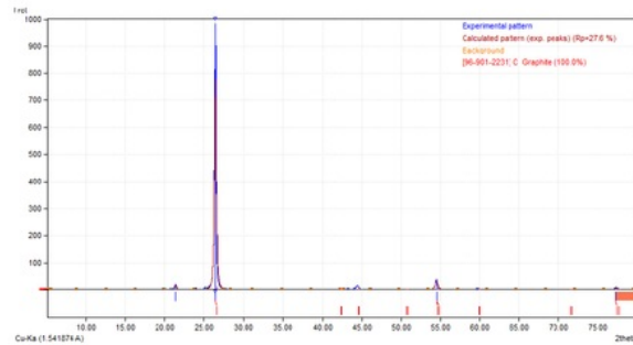
FIG. 2. Diffractogram of graphite 300 mesh.
