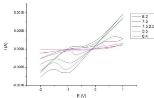
FIG. 7. Voltammogram by determining optimum composition of GO:paraffin.
